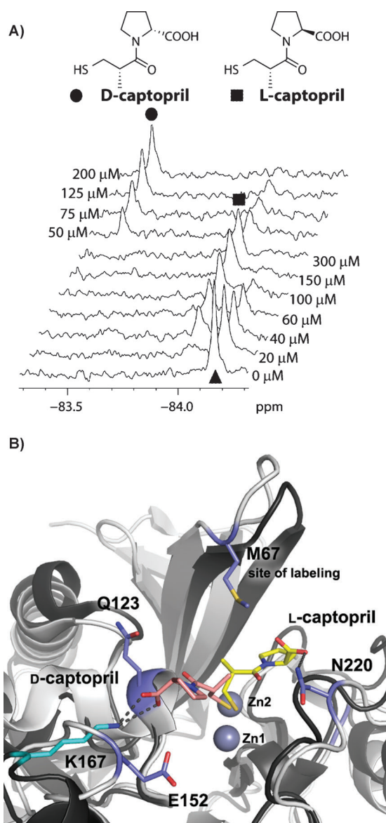
Figure 2. Monitoring of inhibitor binding to NDM-1 MBL by ^{19}\text{F} NMR spectroscopy. A) Titration of NDM-1*·di- \text{Zn}^{\text{II}} (▲) with captopril stereoisomers leads to the appearance of distinctive peaks attributed to L- (■) and D-captopril (●) complexes. L-Captopril can be displaced from a NDM-1* by D-captopril. B) The different chemical shifts for L- and D-captopril likely reflect different binding modes. View from crystallographic analyses of NDM-1 complexed with di- \text{Zn}^{\text{II}} and L-captopril (PDB id: 4EXS). The L-captopril (yellow) interacts with Asn220. Binding of D-captopril (pink) is modeled based on a structure of D-captopril complexed with the BlaB MBL (PDB id: 1M2X).
